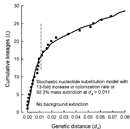
Fig. 4. Model of lineage accumulation with relative age in which genetic distance is estimated by a stochastic model of nucleotide substitution with a change in the colonization rate at B = 0.011 . The apparent colonization rates are 1705 ( A < B ) and 131 ( A > B ). The genetic distance scale extends only to 0.08 to emphasize the fit to the more recent accumulation of lineages.
